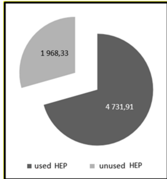
Fig. 2 Usage of technical HEP - production [GWh/year] (own processing based on VÚVH data)
